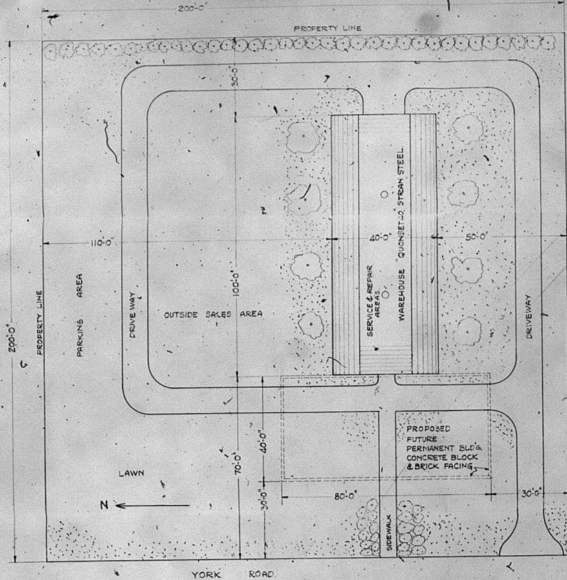
PLOT PLAN SCALE \frac{1}{4}" = 1 \text{ FOOT}
