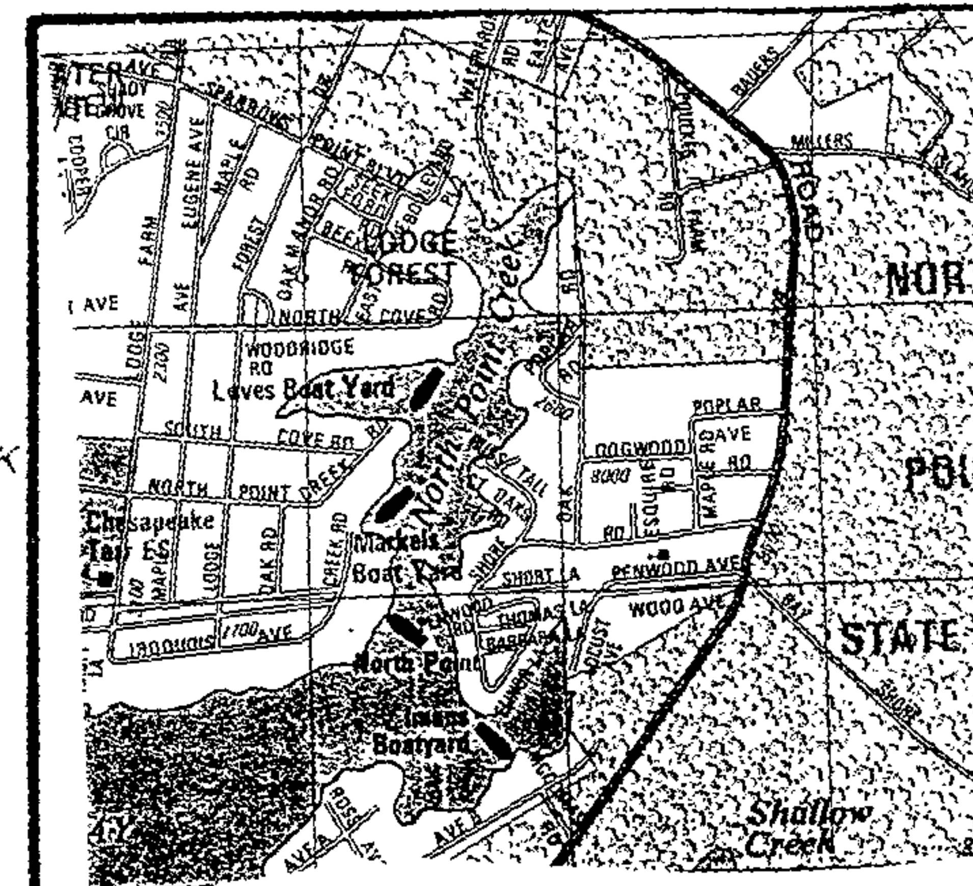
VICINITY MAP
