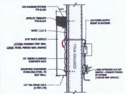
CHANNEL LETTER & LOGO DETAIL SCALE: NTS
