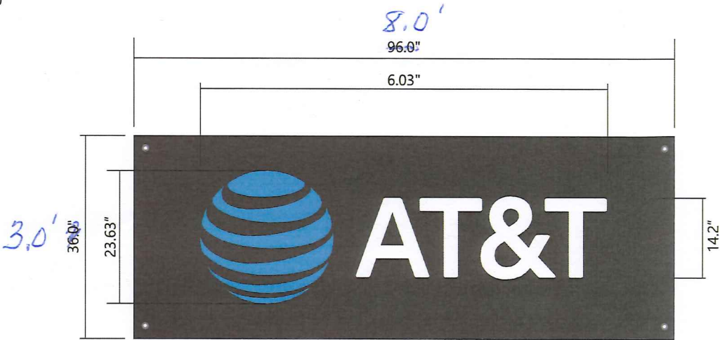
FRONT VIEW SCALE: 1/2" =1'-0"
